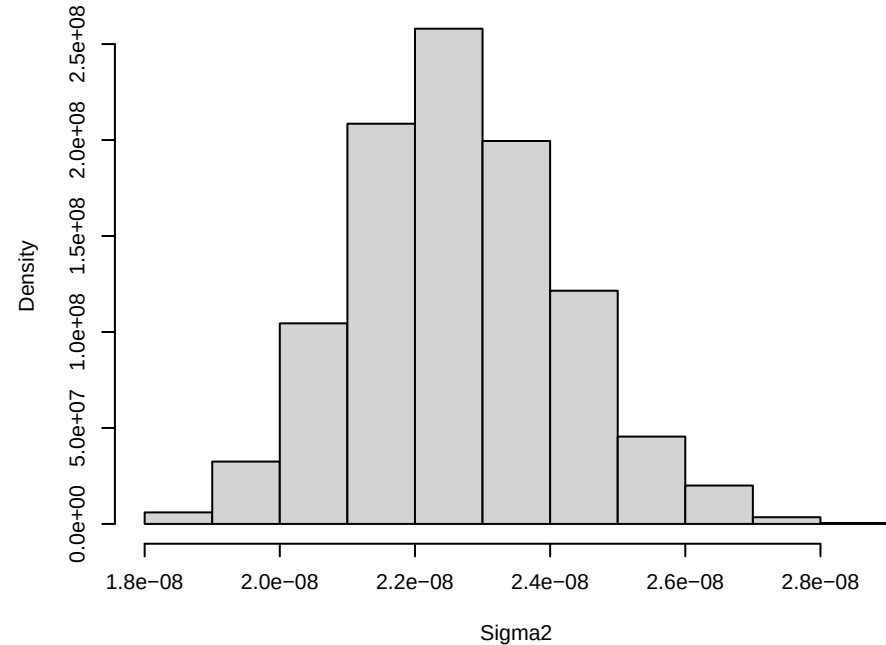
Density of Sigma2
